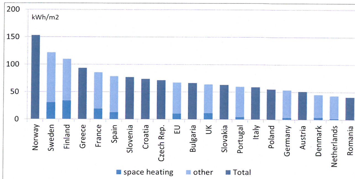
Fig. 4.2. Consumul specific de energie electrica in locuinte ( \text{KWh/m}^2 )
